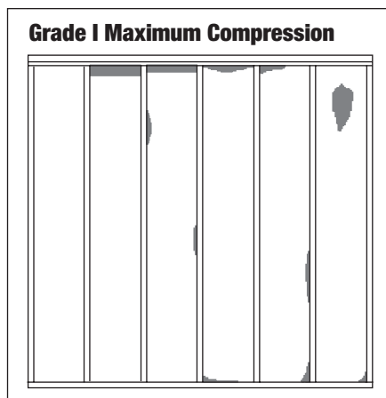
Figure 2. The gray shading shows insulation compression or incomplete fill of approximately 2%.
