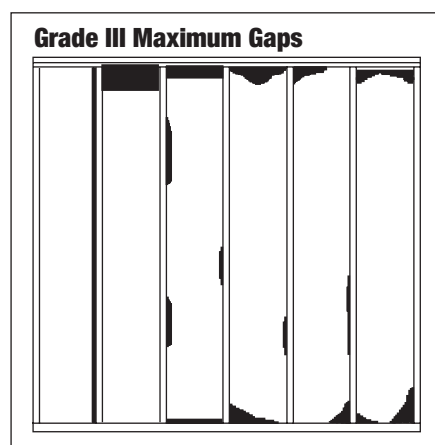
Figure 5. The black shading represents insulation gaps of approximately 5%.
