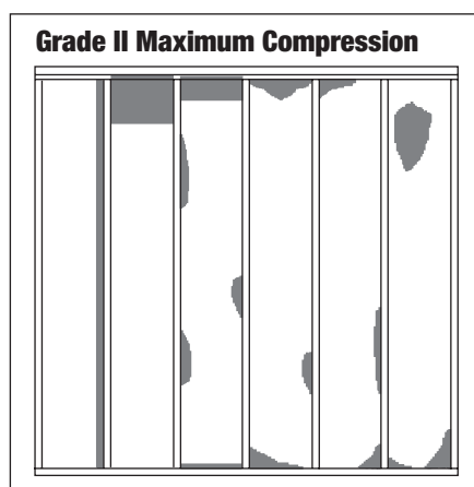
Figure 4. The gray shading represents insulation compression or incomplete fill of approximately 10%.
