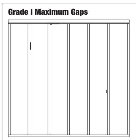
Figure 1. Occasional very small gaps are acceptable for "Grade I."
