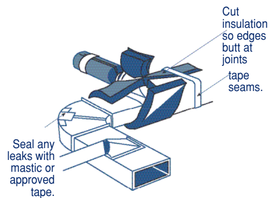
Figure 20: Re-tighten and seal leaky ducts before insulating with foil-faced batts. Tape seams with mastic tape.
