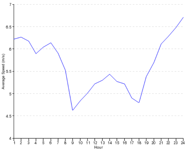
71m W Diurnal Wind Speed
