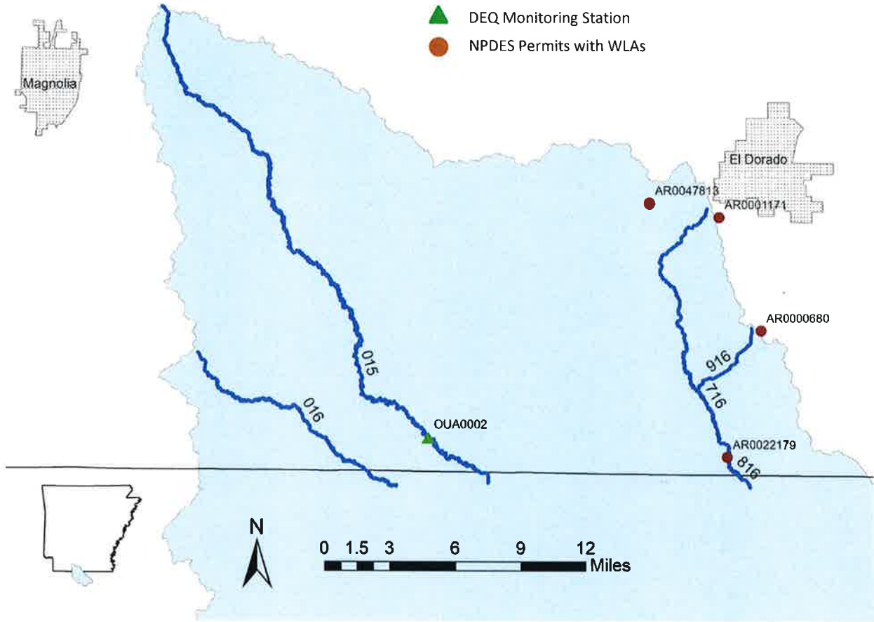
Figure 1: Map of Upper Cornie Bayou AUs with affected permits and DEQ monitoring station OUA0002 depicted.
