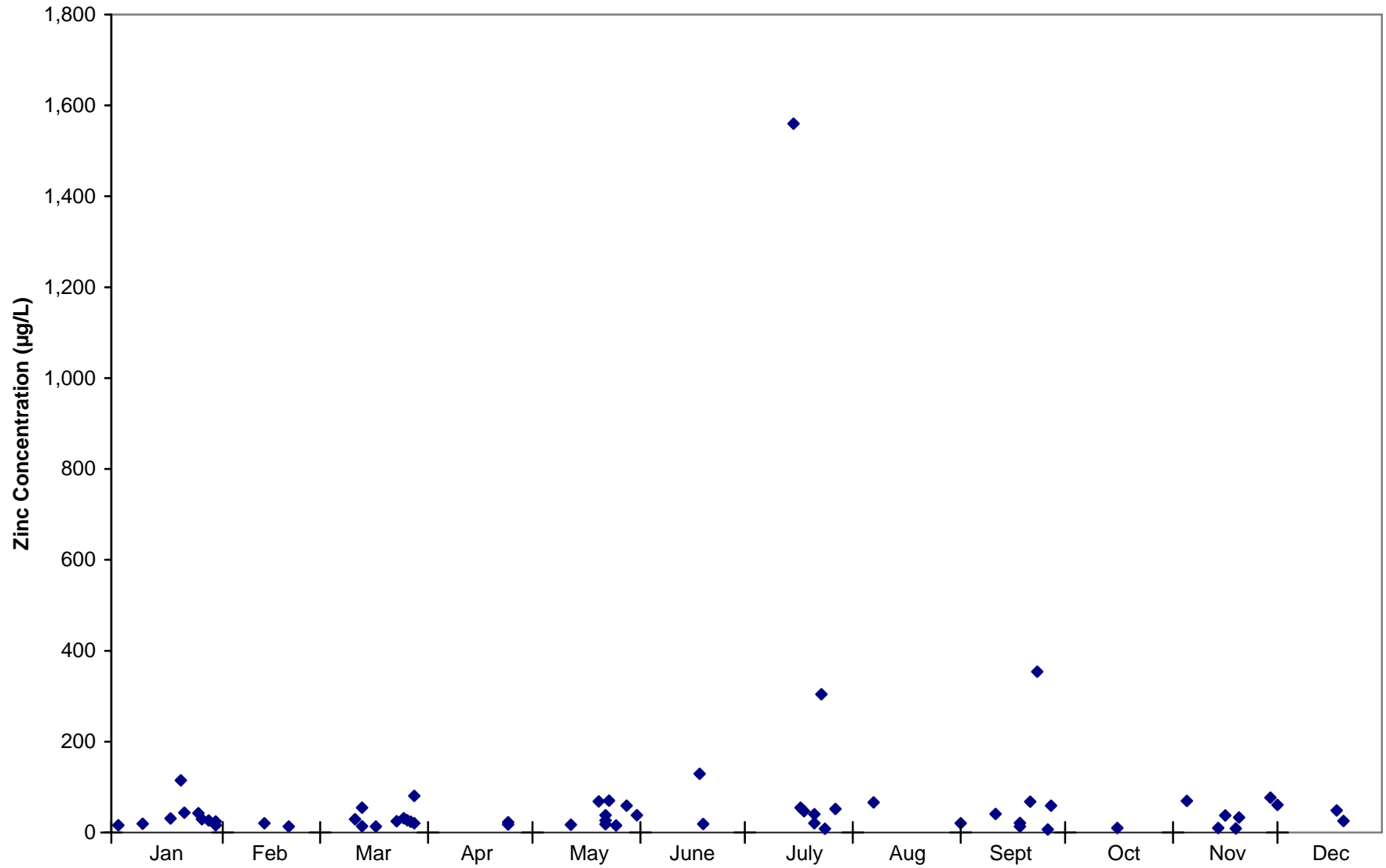
Figure B.4. Seasonal Plot of Zinc in Big Cornie Bayou near Three Creeks (OUA0002)
