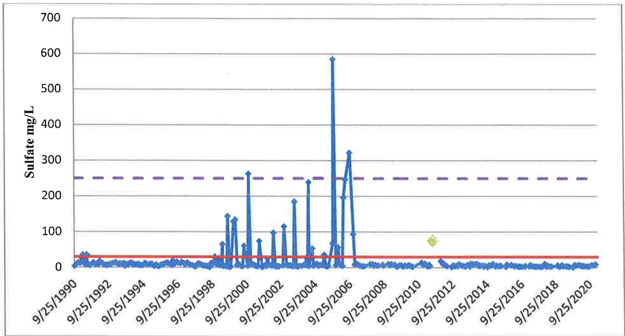
Figure 2: Sulfate data for OUA0002 located on AU AR_08040206_015 from 1990-2020. The solid line represents the site specific criterion of 30 mg/L for sulfates. The dashed line represents the 250 mg/L domestic water supply criterion. The large diamond represents the date the TMDL was approved.
