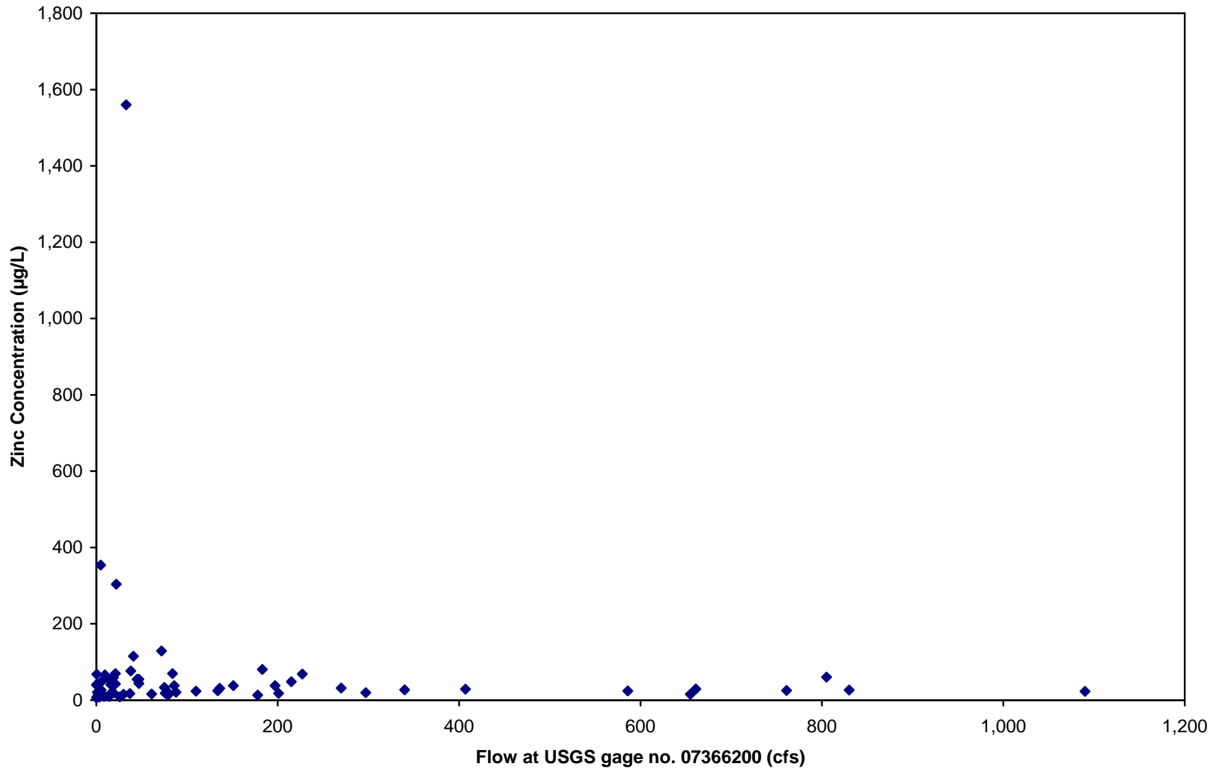
Figure B.6. Zinc vs flow for Big Cornie Bayou near Three Creeks (OUA0002)
