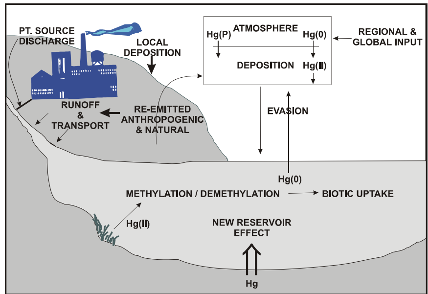
Figure 4.1. General mercury cycle showing atmospheric transport and deposition, point, nonpoint source and natural background contributions, and the effects of new reservoirs on mercury release into the environment (after Mason et al. 1994).
