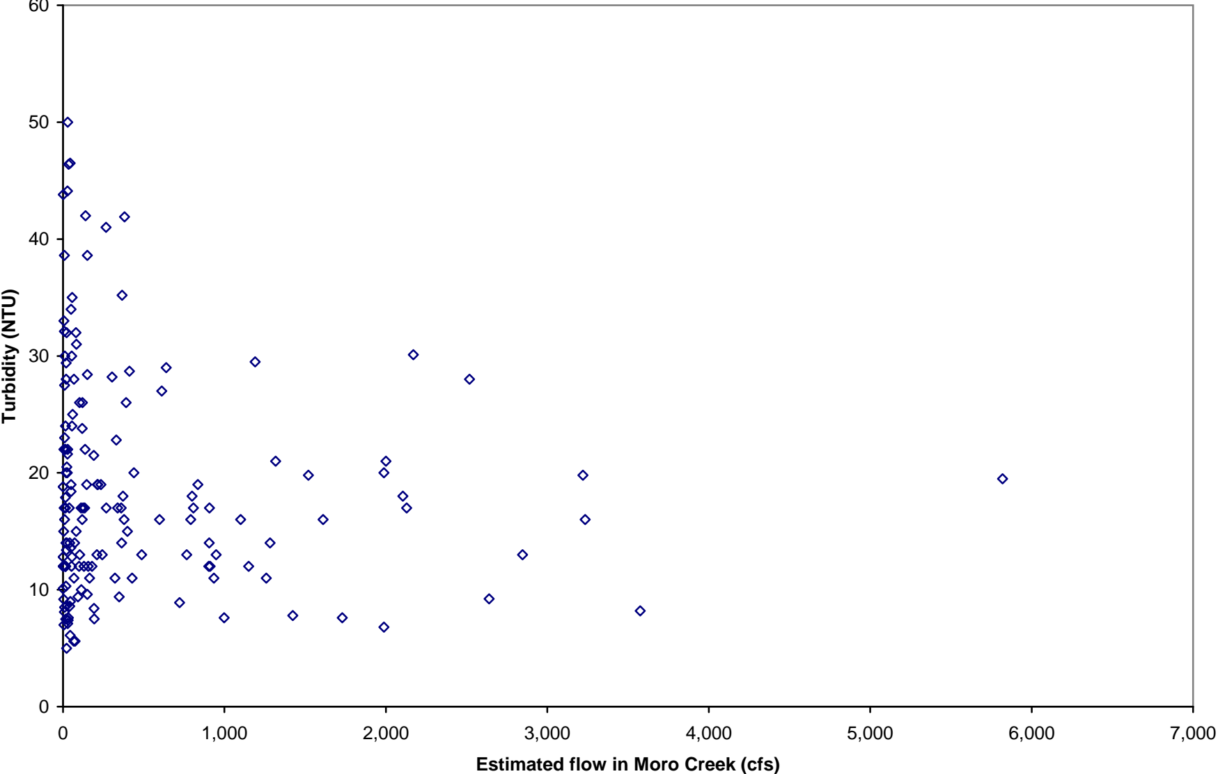
Figure C.18. Turbidity vs Flow for Moro Creek (OUA0028)
