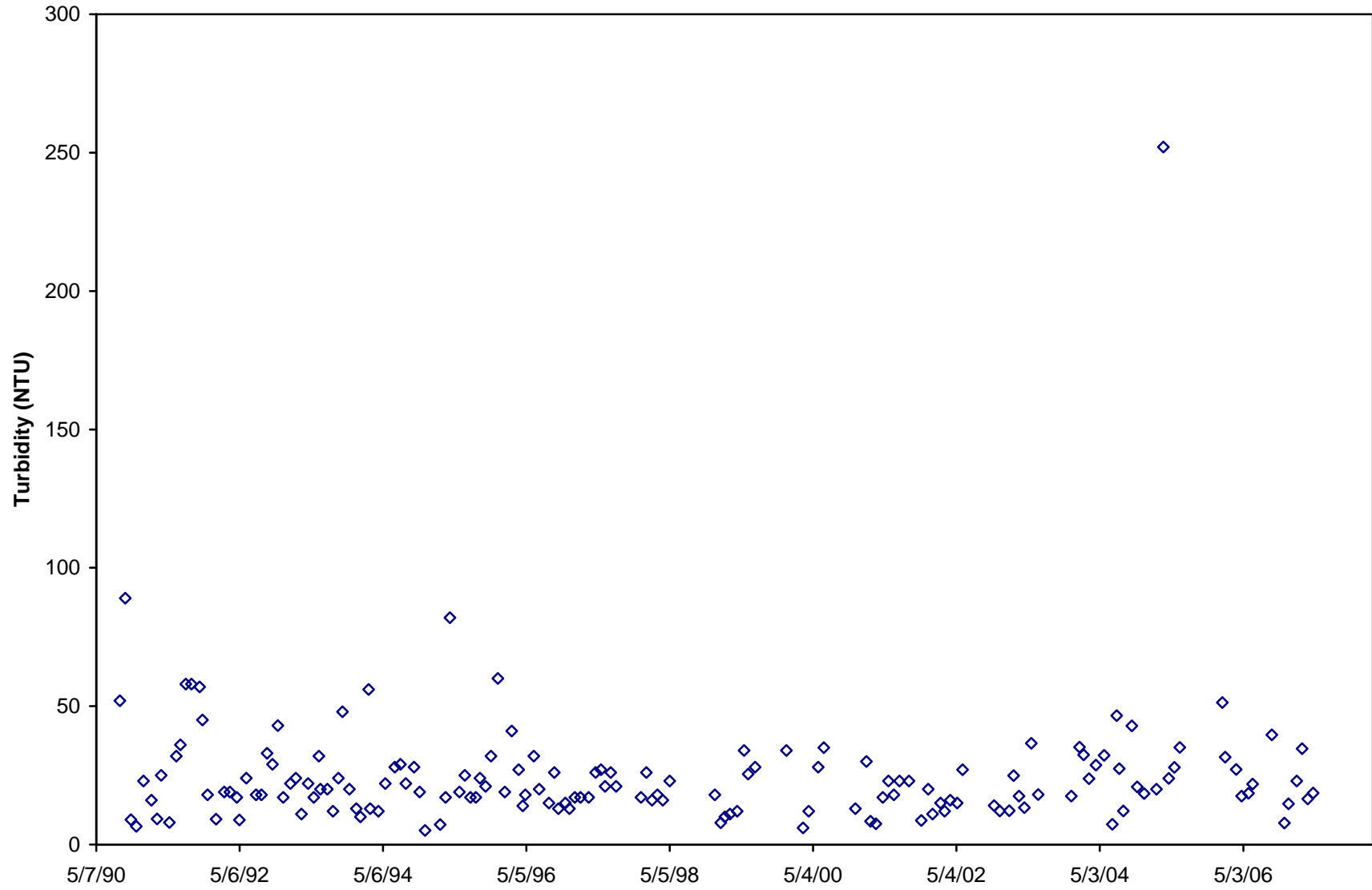
Figure C.1. Time Series Plot of Turbidity for Big Creek near Pansy (OUA0043)
