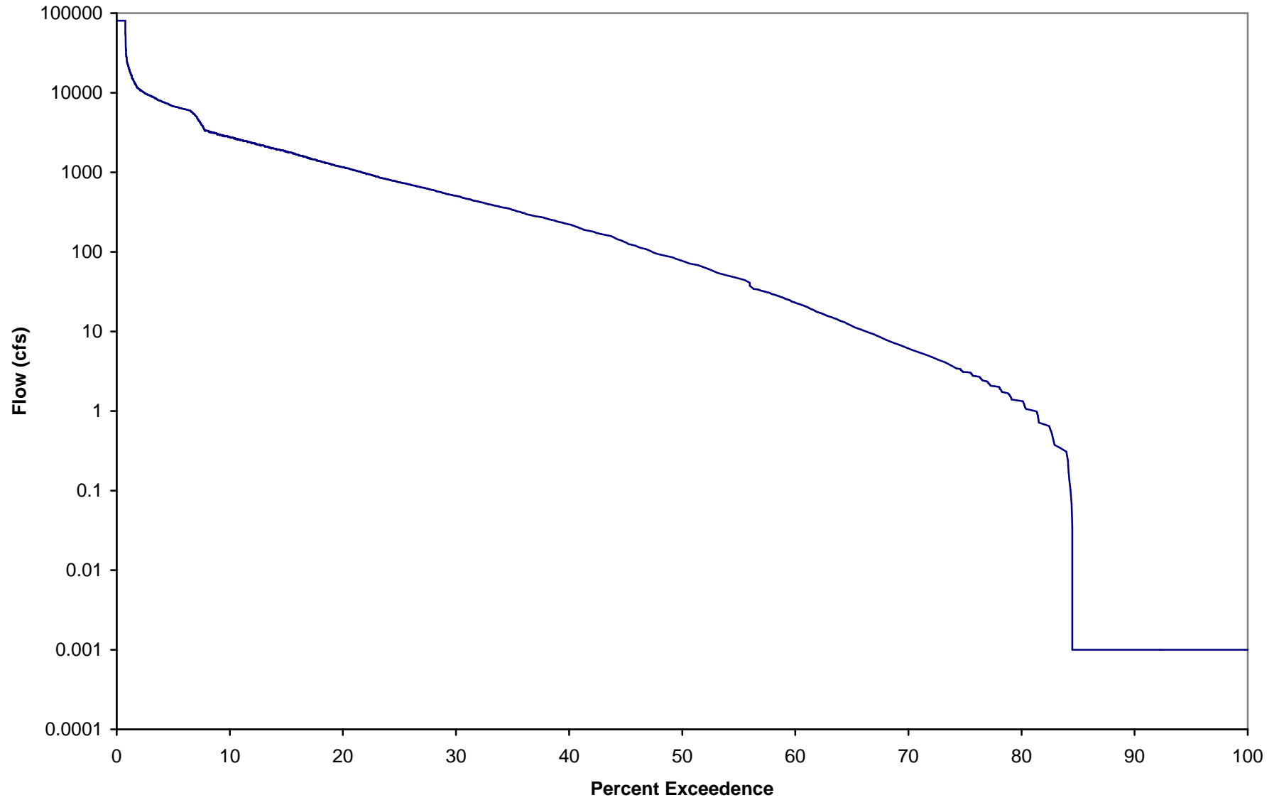
Figure I.1. Flow duration curve for Moro Creek (08040201-001L)
