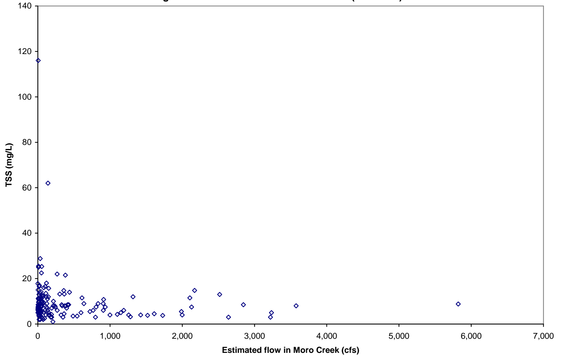
Figure C.22. TSS vs Flow for Moro Creek (OUA0028)
